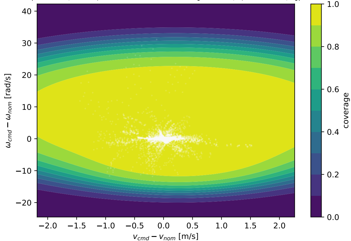
Residual coverage vs command offset (0 = off / OOD; state fixed at mean [0.40 m/s, 0.07 rad/s])
